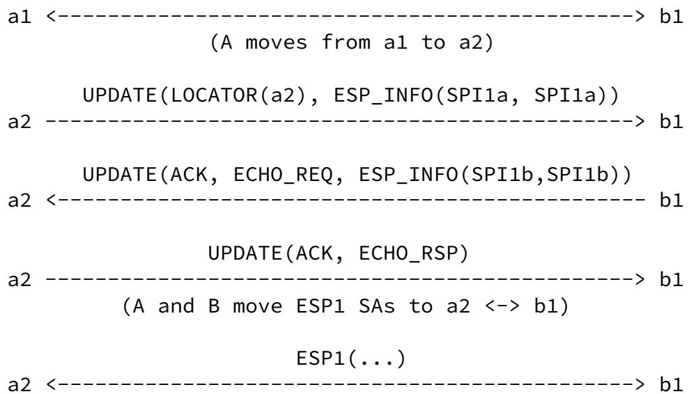
Figure 3: Break Before Make
