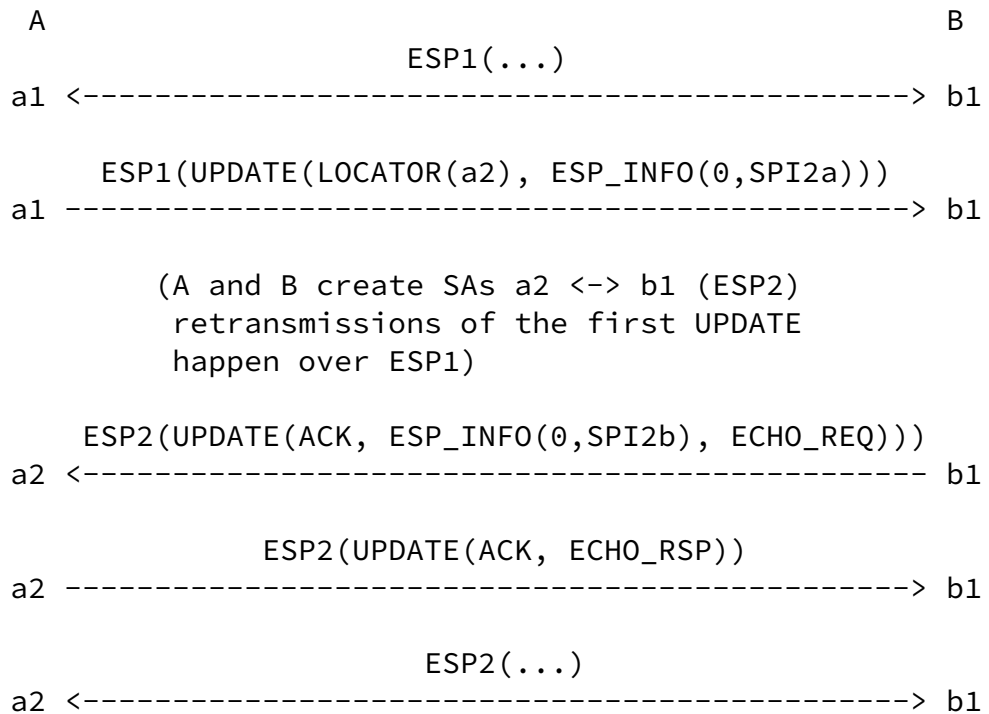
Figure 2: Make Before Break
