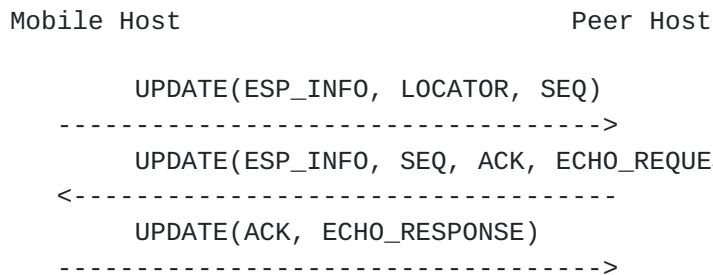
Figure 3: Readdress without Rekeying, but with Address Check
