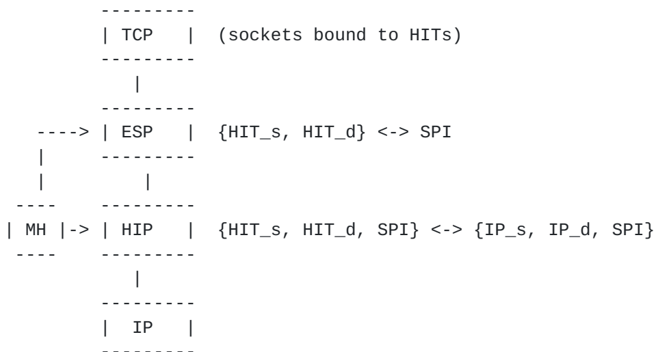
Figure 2: Architecture for HIP Mobility and Multihoming (MH)
