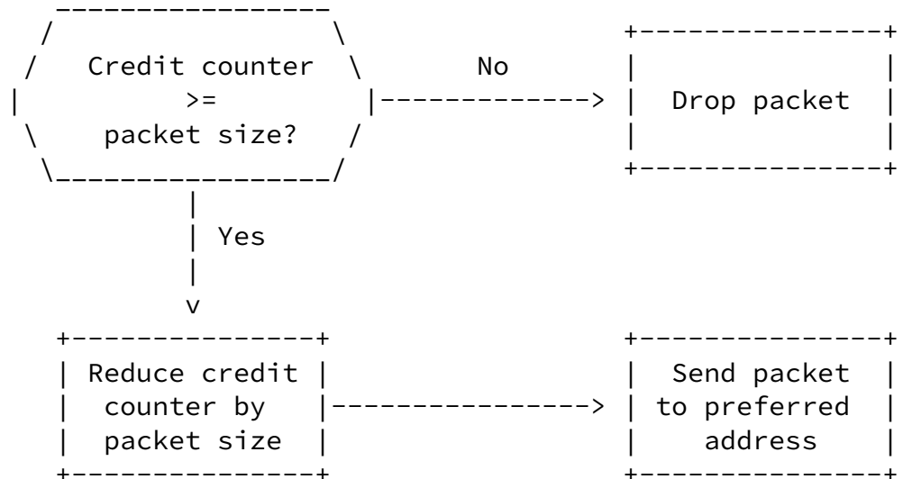
Figure 15: Sending Packets with Credit-Based Authorization
