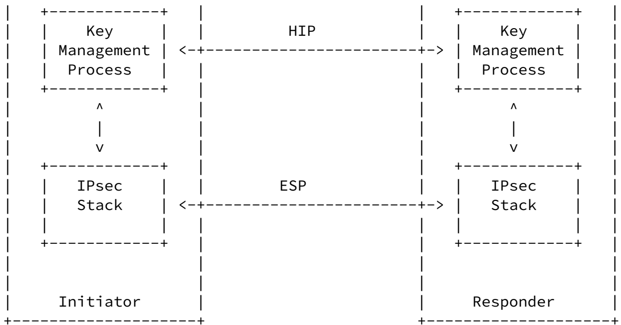
Figure 1: HIP Deployment Model
