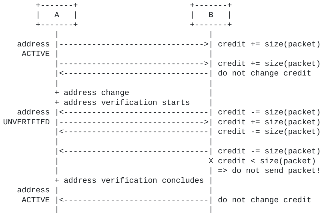
Figure 5: Readdressing Scenario
