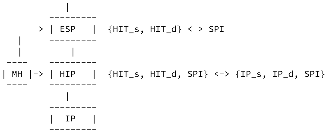
Figure 2: Architecture for HIP Host Mobility (MH)
