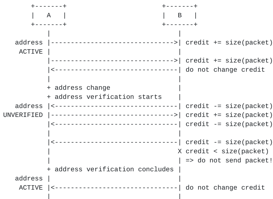
Figure 5: Readdressing Scenario
