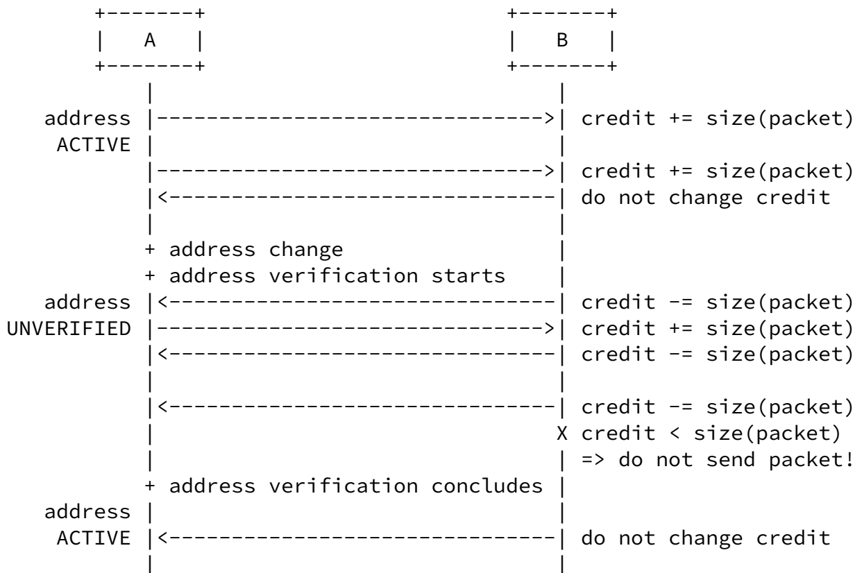
Figure 5: Readdressing Scenario
