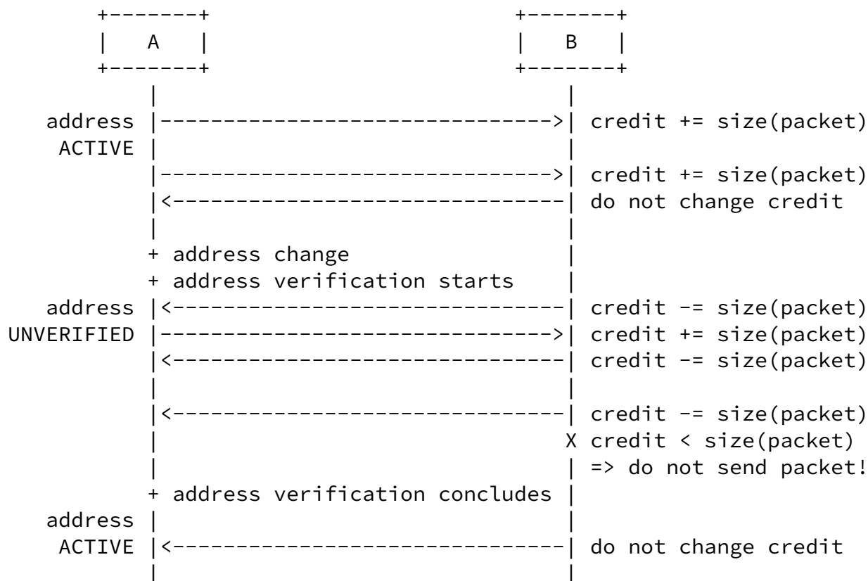
Figure 5: Readdressing Scenario
