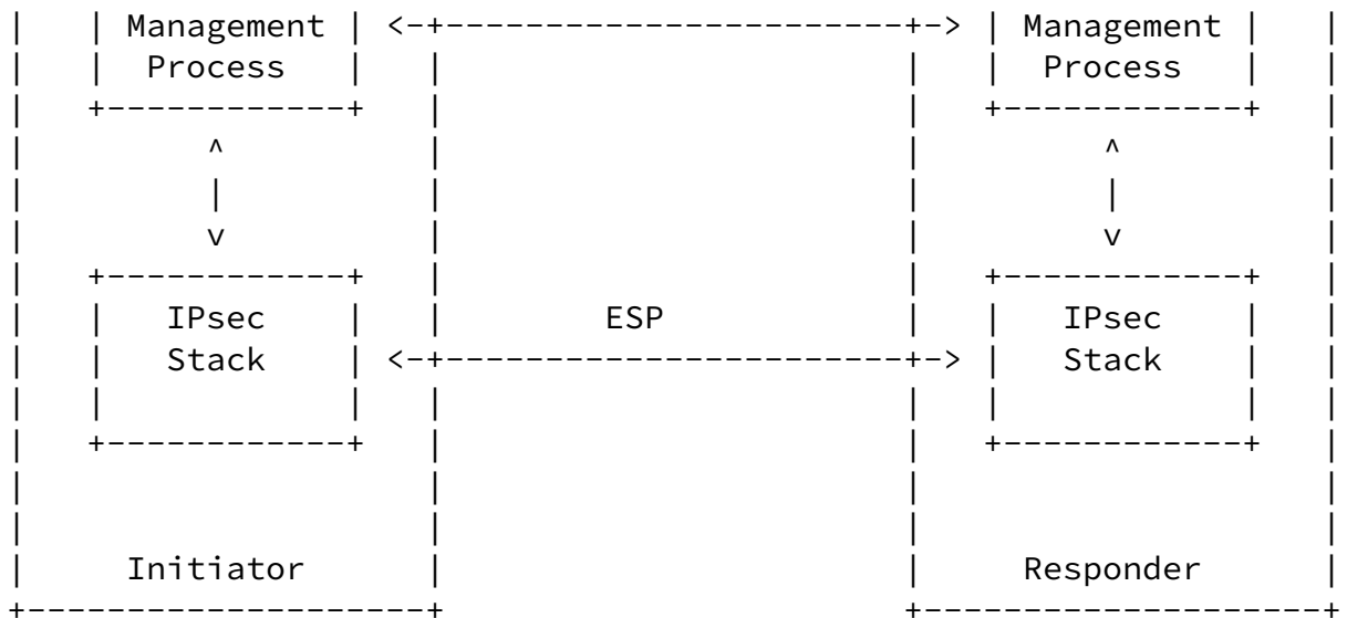
Figure 1: HIP Deployment Model
