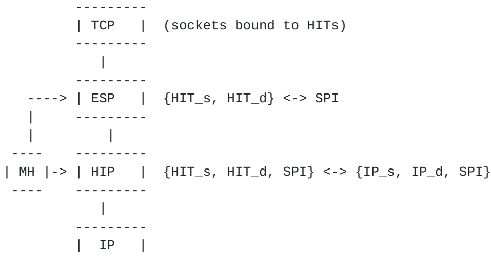
Figure 2: Architecture for HIP Host Mobility (MH)
