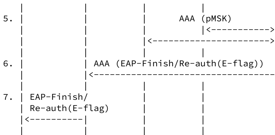
Figure 1: ERP/AAK Operation
