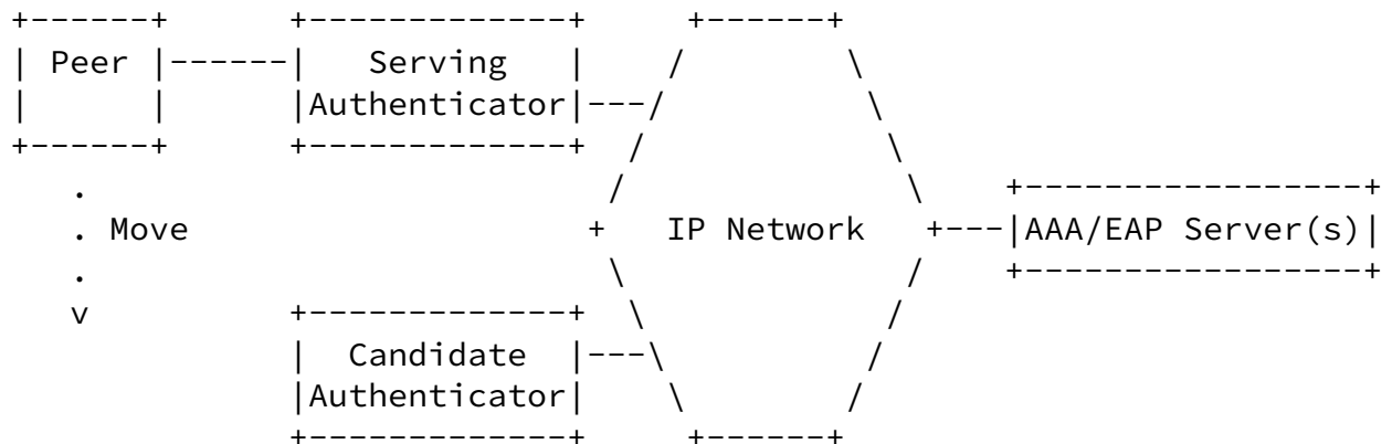
Figure 1: EAP Pre-authentication Functional Elements
