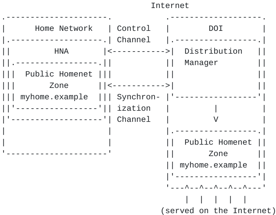
Figure 1: High level architecture overview of outsourcing the Public Homenet Zone
