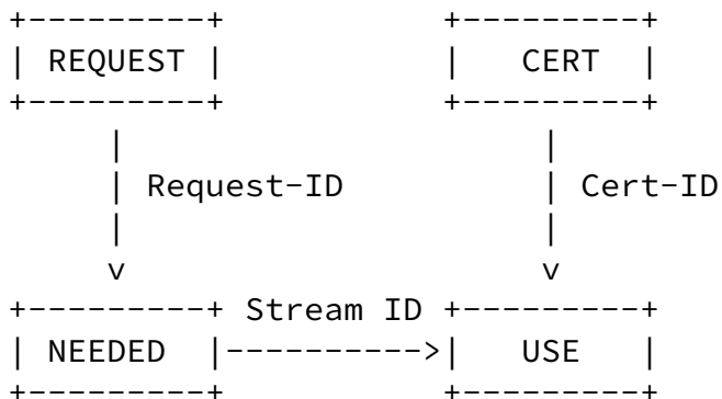
Figure 7: Frame correlation
