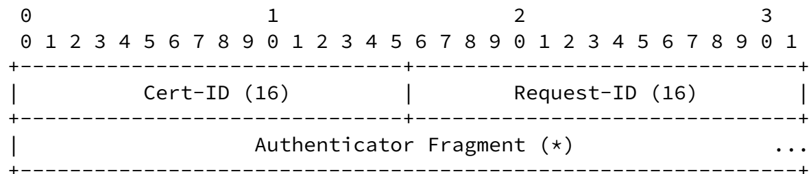
Figure 11: CERTIFICATE frame payload
