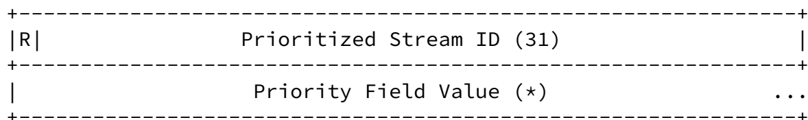
Figure 1: HTTP/2 PRIORITY_UPDATE Frame Payload
