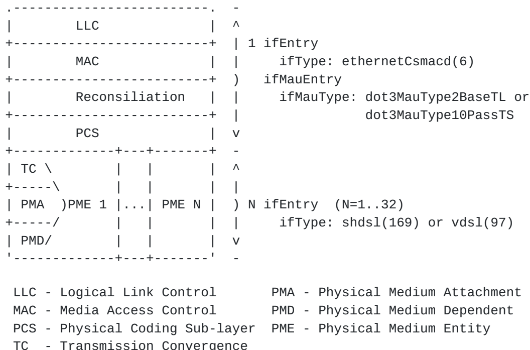
Figure 2: Use of ifTable and ifMauTable for EFMCu ports
