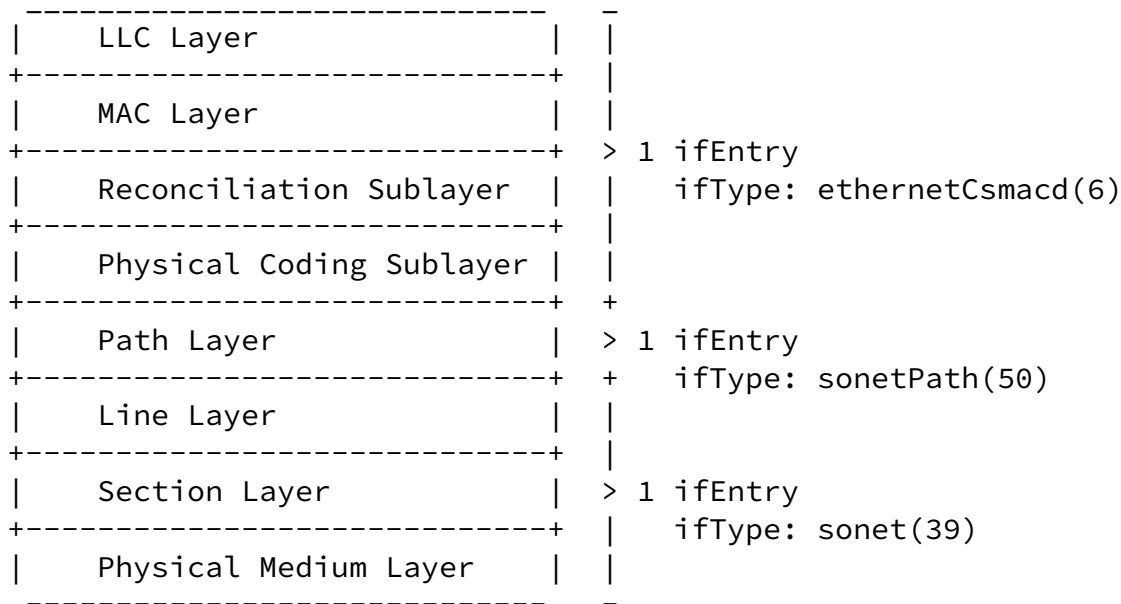
Figure 1 - Use of ifTable for an Ethernet WIS port
