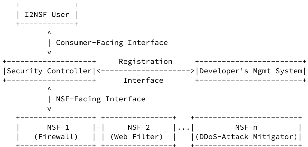
Figure 1: I2NSF Framework
