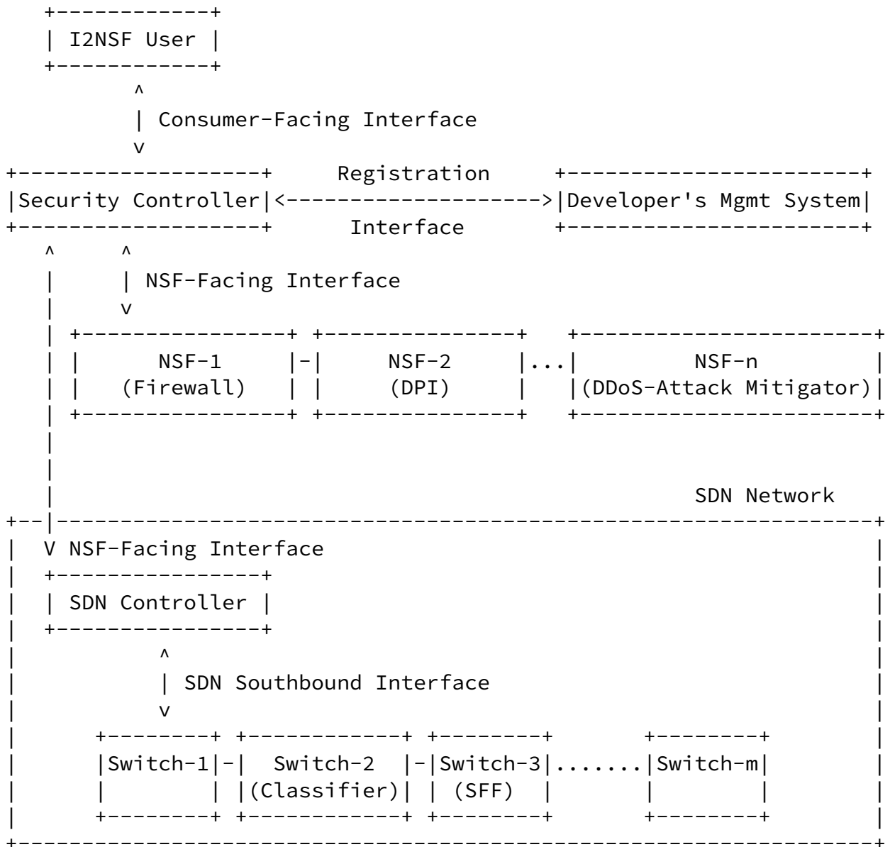
Figure 3: An I2NSF Framework with SDN Network
