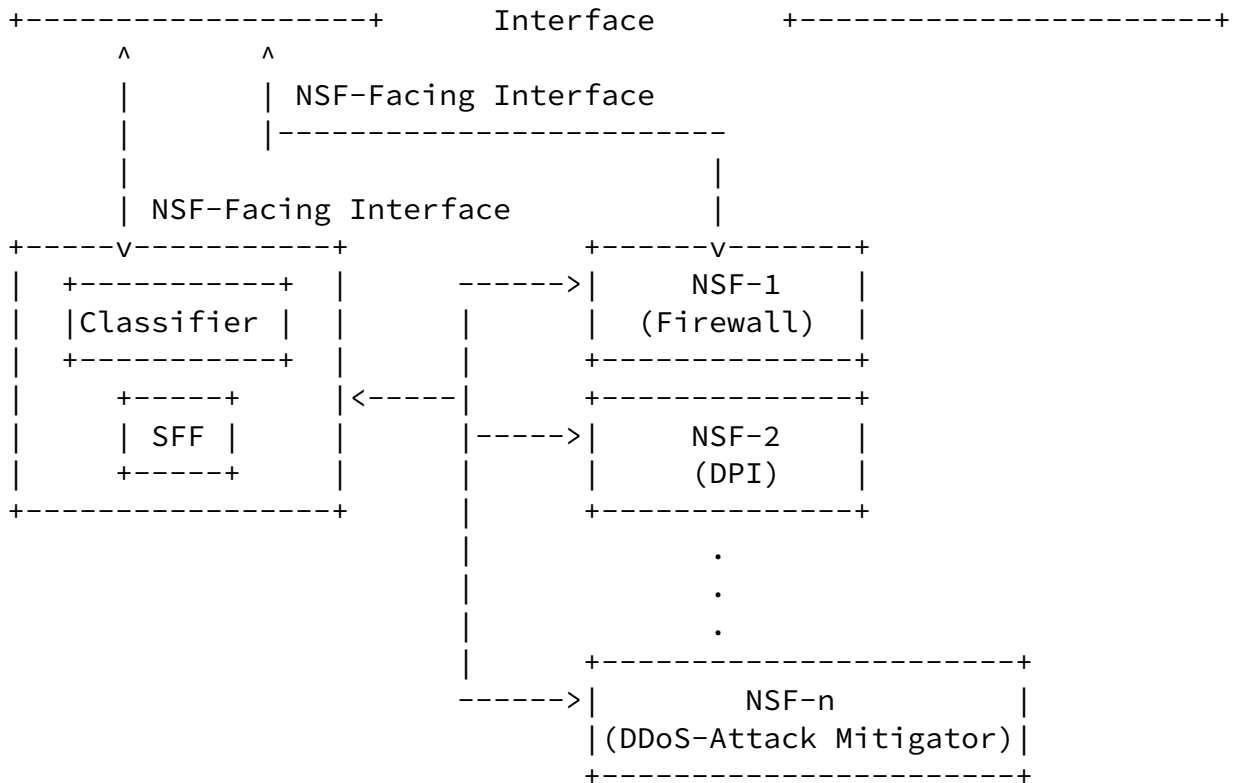
Figure 2: An I2NSF Framework with SFC
