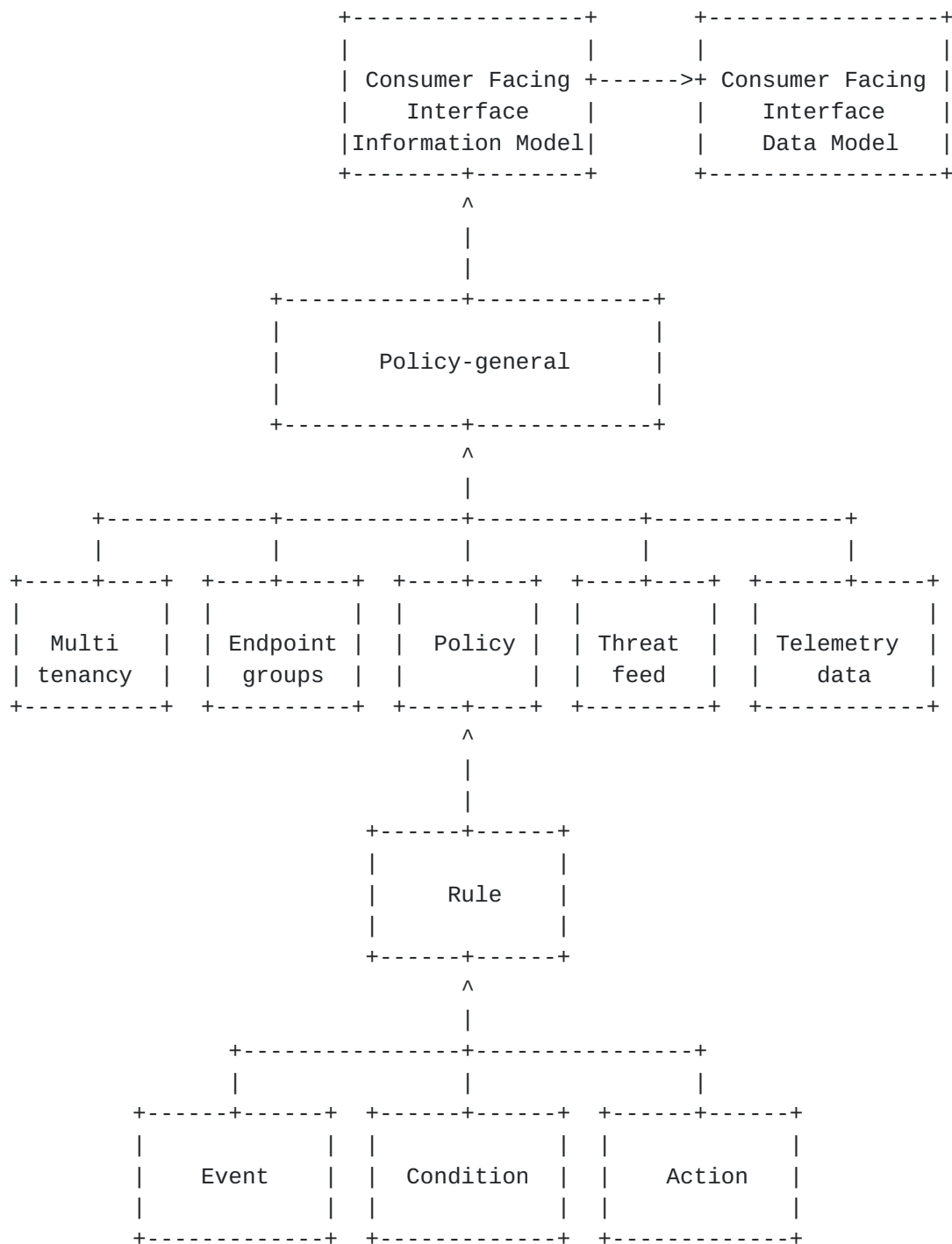
Figure 1: High-level-abstraction for Consumer Facing Interface
