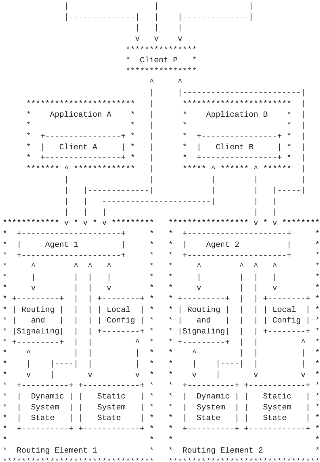
Figure 1: Architecture of I2RS clients and agents
