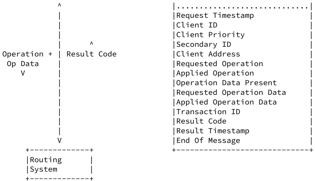
Figure 1: I2RS Interaction Trace Log Capture
