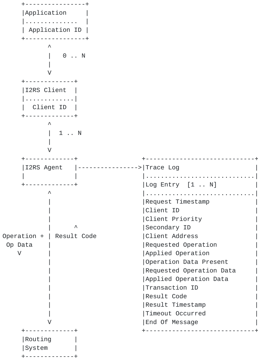
Figure 1: I2RS Interaction Trace Log Capture
