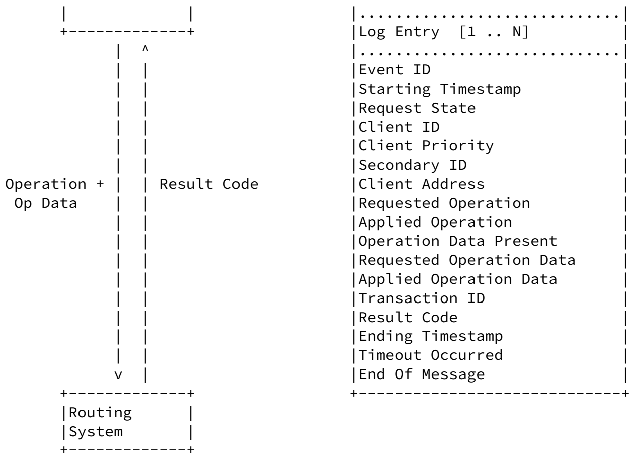
Figure 1: I2RS Interaction Trace Log Capture
