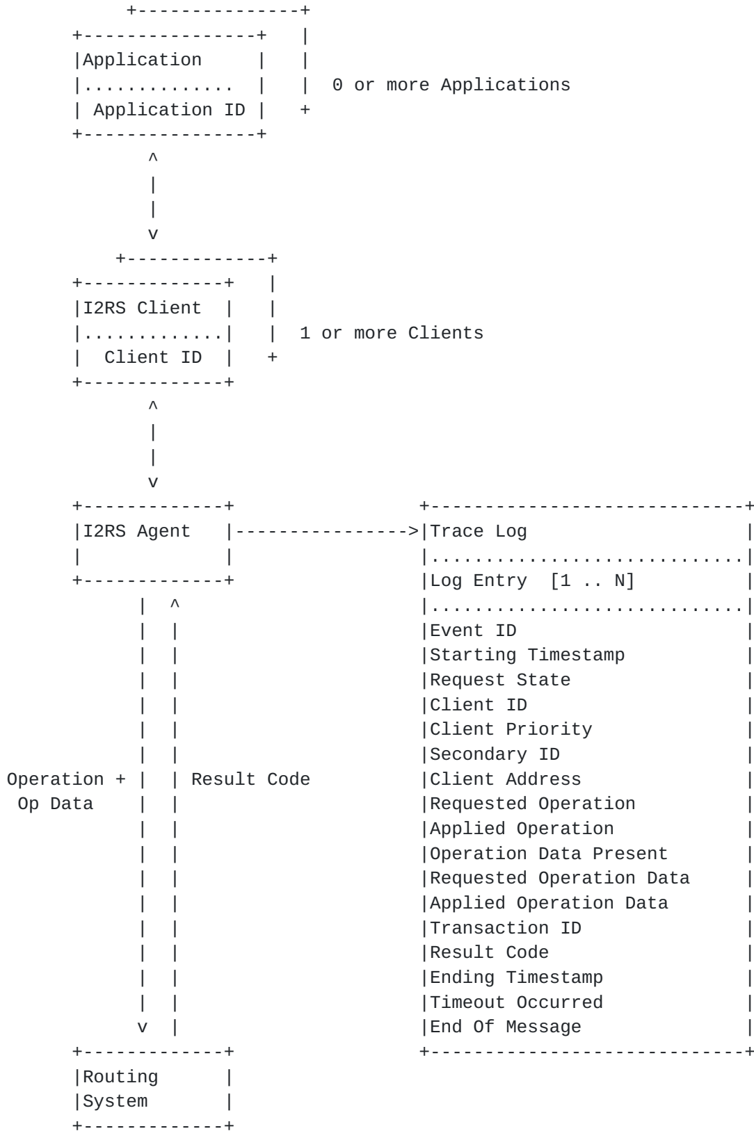
Figure 1: I2RS Interaction Trace Log Capture
