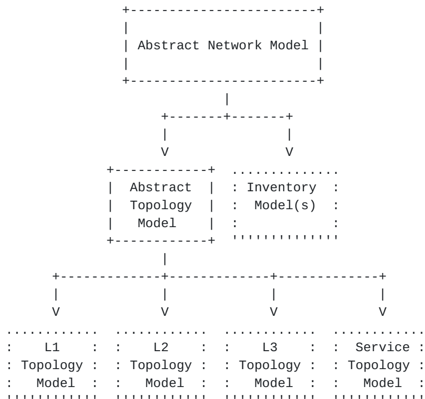
Figure 1: The network data model structure
