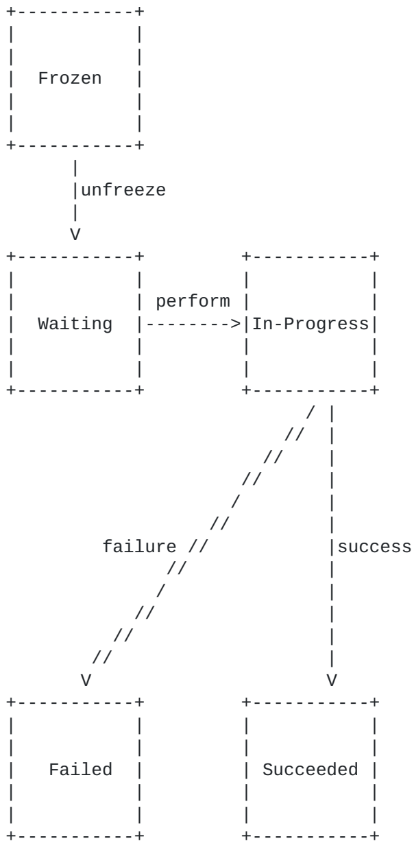
Figure 8: Pair State FSM
