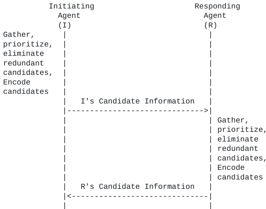
Figure 6: Candidate Gathering and Exchange Sequence
