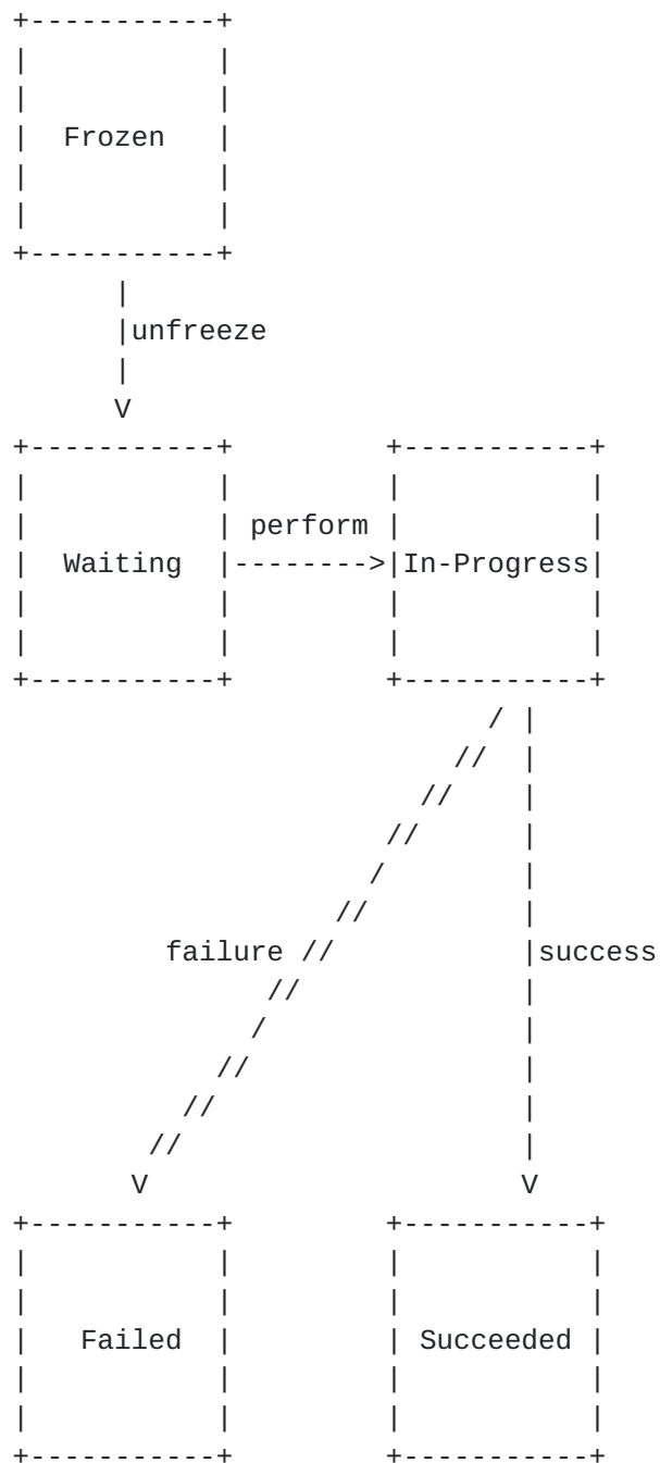
Figure 6: Pair State FSM
