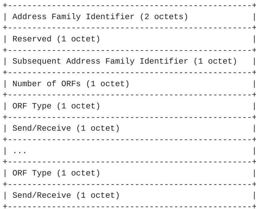
Fig 4. Capability encoding
