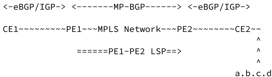
Figure 1 MPLS VPN Network
