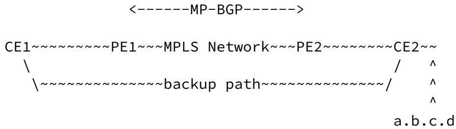
Figure 3 MPLS VPN Network - CE1-CE2 Backup connection
