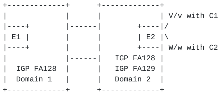
Figure 11: BGP CAR resolution over IGP FLeX-Algo for resource avoidance in a domain
