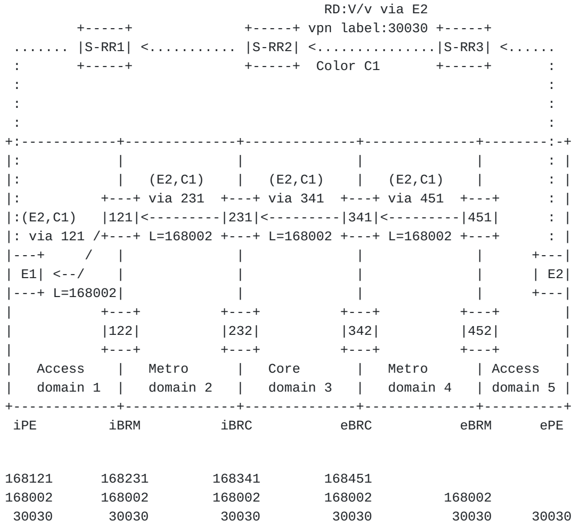
Figure 3: Flat Transport Network Design
