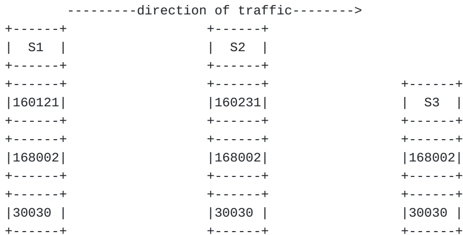
Figure 7: BGP SR policy Aware transport CAR path
