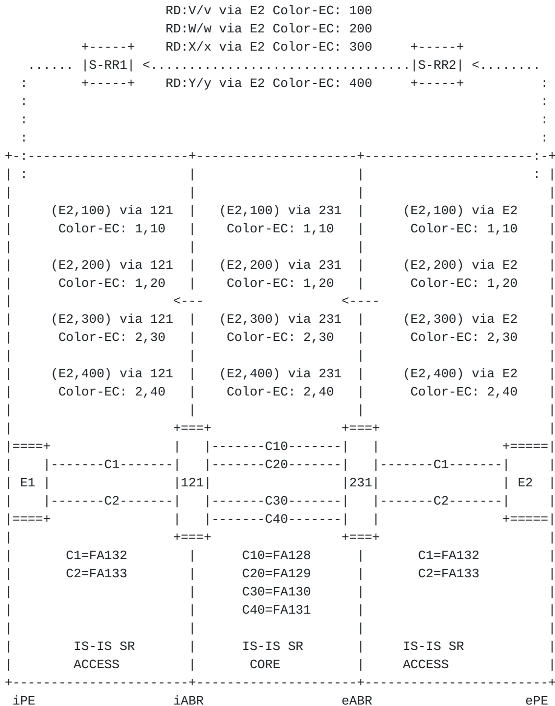
Figure 13: N:M illustration
