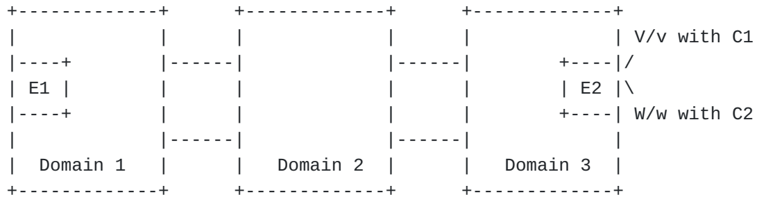
Figure 1: BGP CAR Solution Illustration
