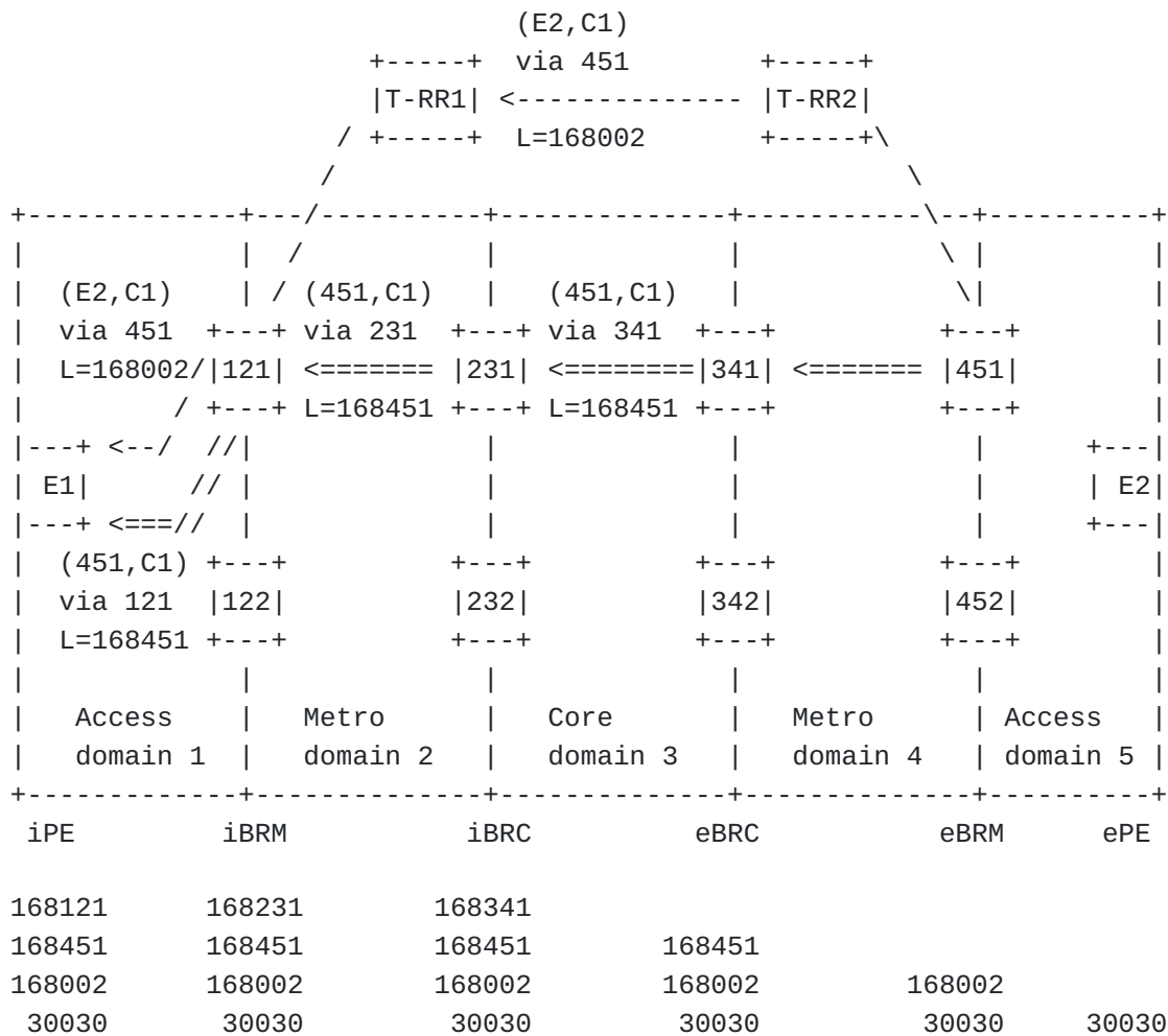
Figure 5: Hierarchical BGP transport CAR, Next-Hop-Unchanged (NHU) at iBR
