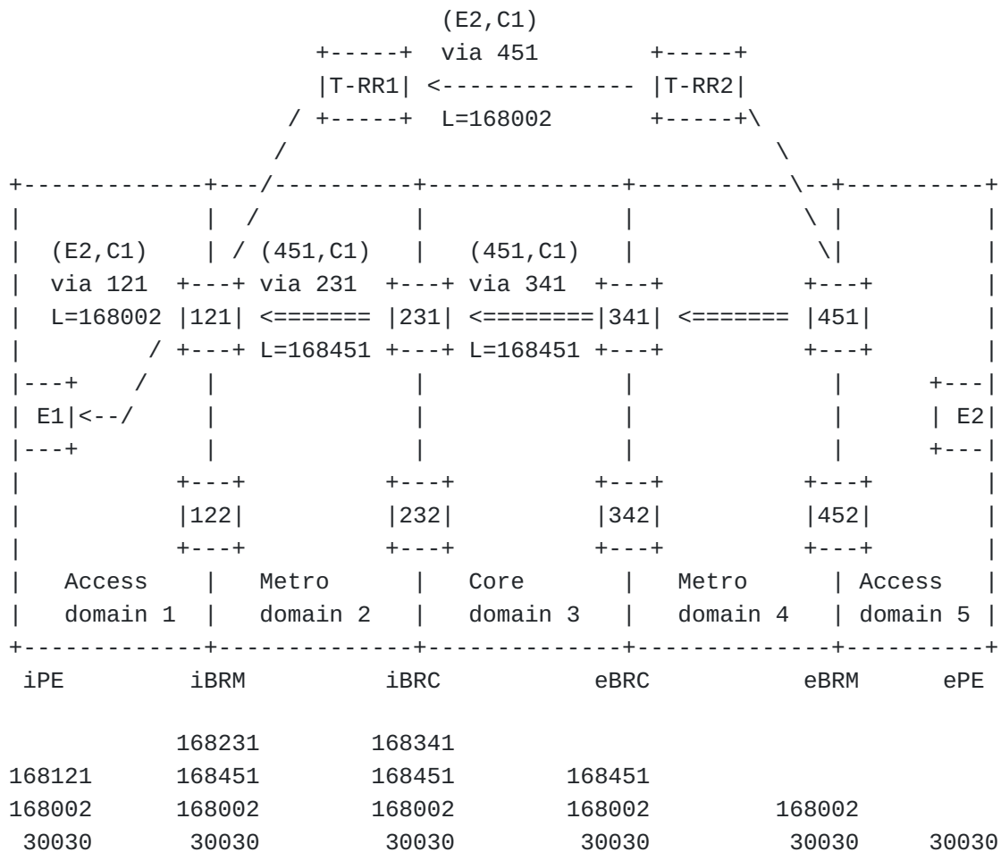
Figure 4: Hierarchical BGP transport CAR, Next-Hop-Self (NHS) at iBR
