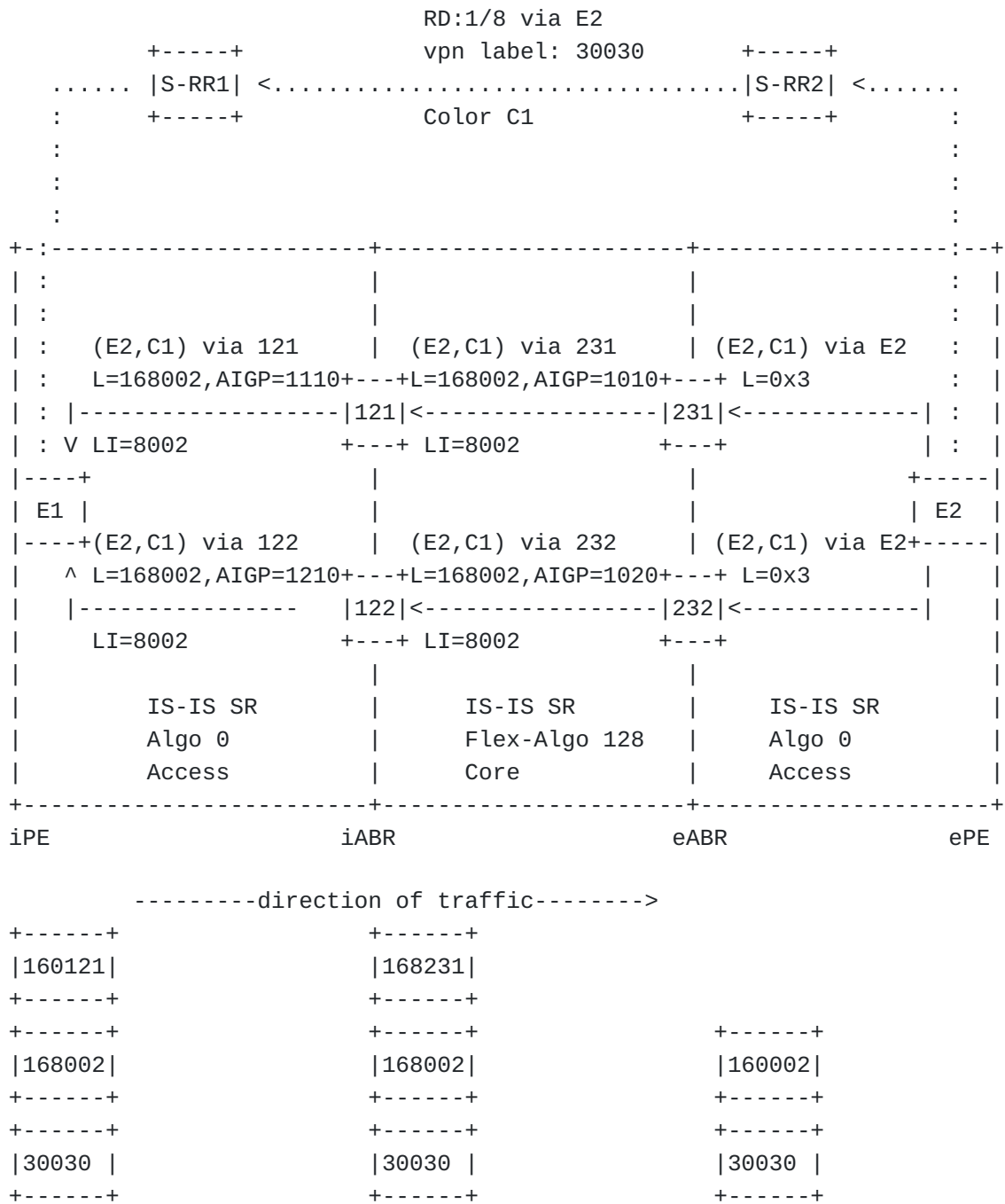
Figure 8: BGP Hybrid Flex-Algo Aware transport CAR path
