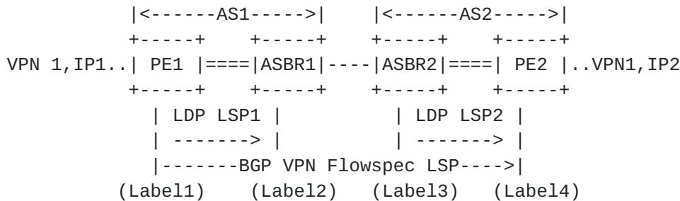
Figure 1: Usage of FlowSpec with Label
