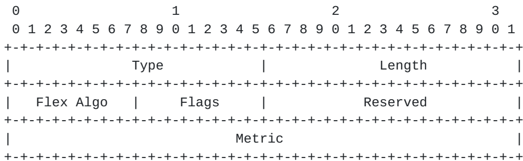
Figure 8: Flexible Algorithm Prefix Metric TLV
