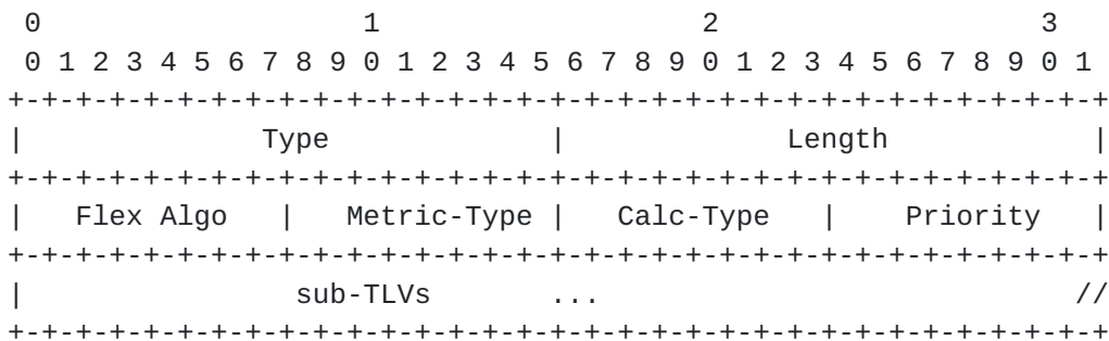
Figure 1: Flexible Algorithm Definition TLV
