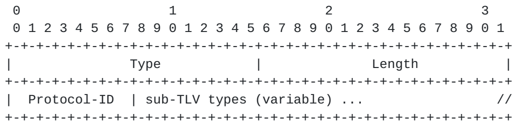
Figure 7: Flexible Algorithm Unsupported sub-TLV
