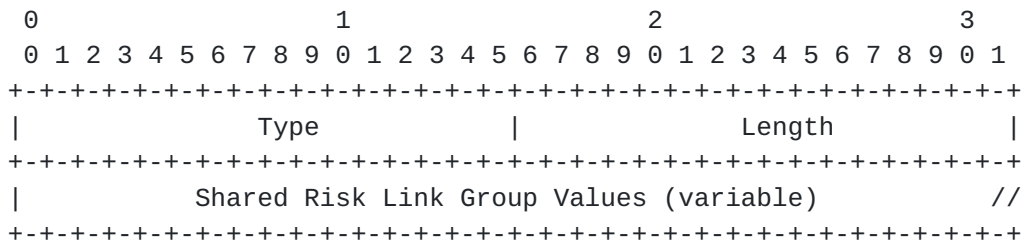
Figure 6: Flexible Algorithm Exclude SRLG sub-TLV
