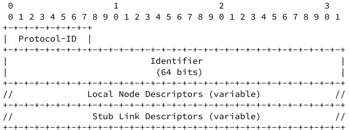
Figure 2: Stub Link NLRI Format
