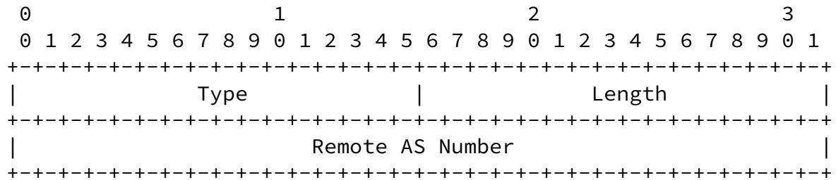
Figure 4: Remote AS Number TLV Format
