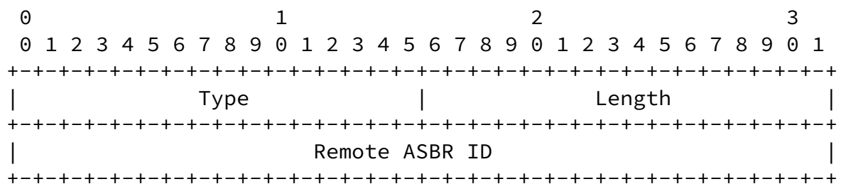
Figure 5: IPv4 Remote ASBR ID TLV Format
