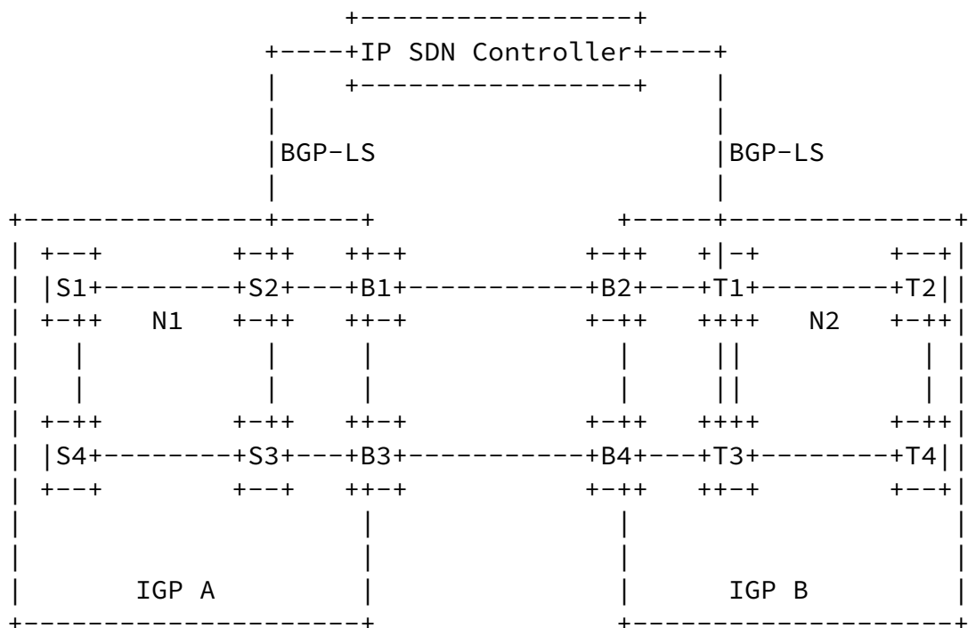
Figure 1: Inter-AS Domain Scenarios
