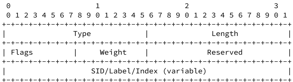
Figure 3: BGP Peering SIDs TLV Format
