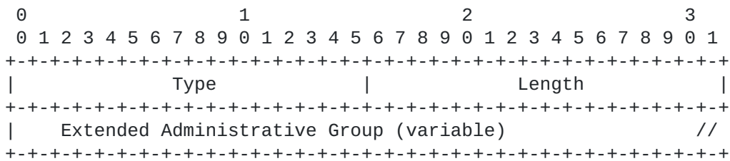
Figure 1: Extended Administrative Group TLV Format
