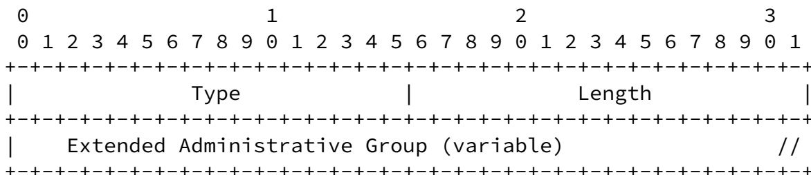
Figure 1: Extended Administrative Group TLV Format
