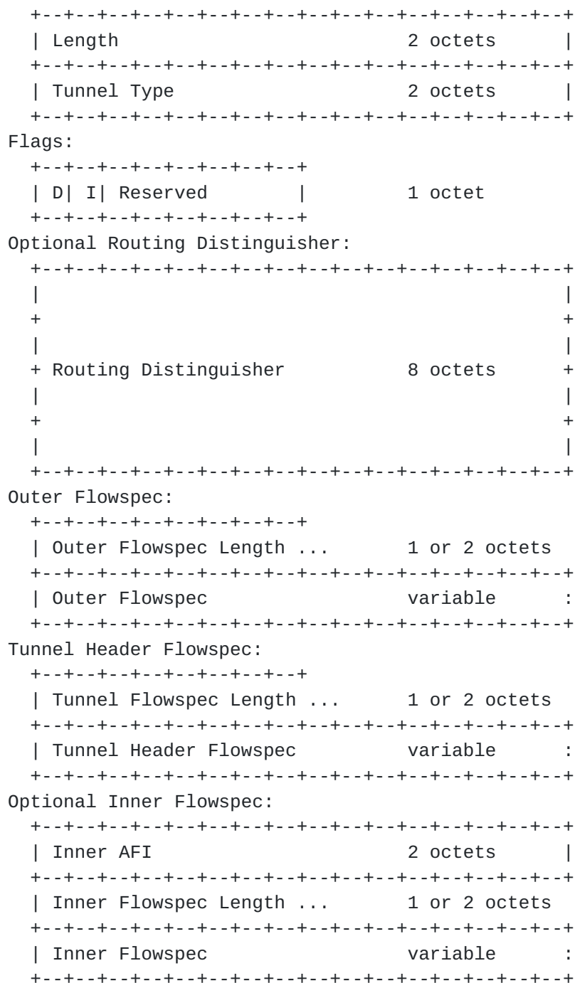
Figure 1. Tunnel Traffic Flowspec NLRI
