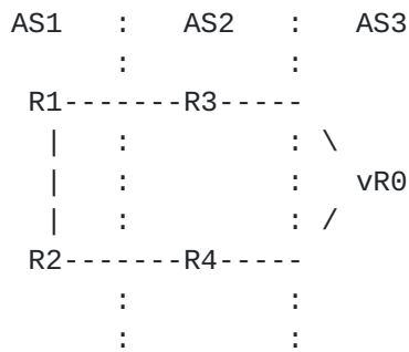
Figure 36: Multi-AS Aggregation
