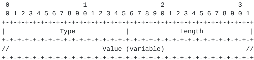
Figure 4: TLV Format
