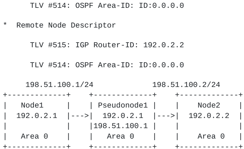
Figure 33: OSPF Pseudonodes
