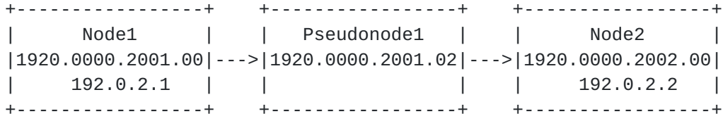
Figure 32: IS-IS Pseudonodes
