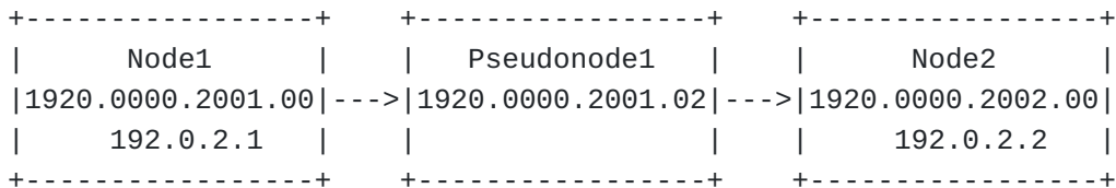
Figure 32: IS-IS Pseudonodes
