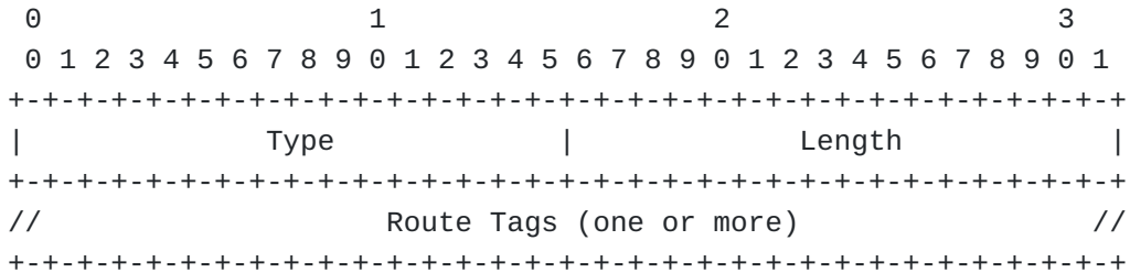
Figure 26: IGP Route Tag TLV Format
