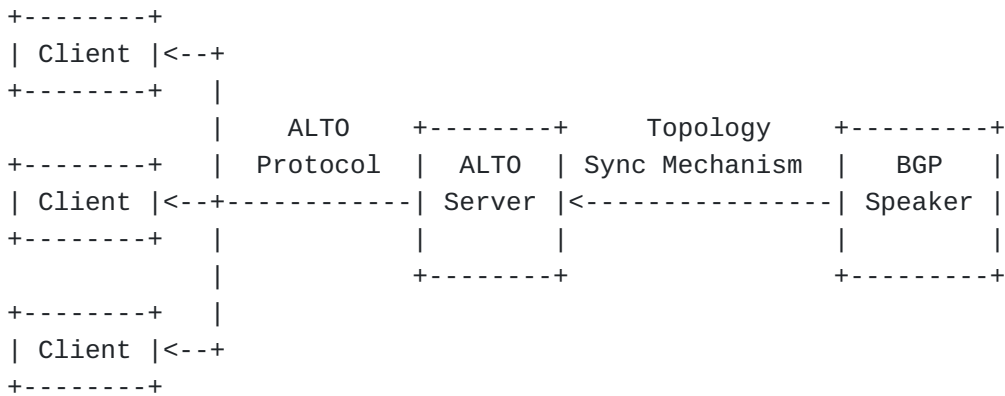
Figure 3: ALTO Server Using Network Topology Information
