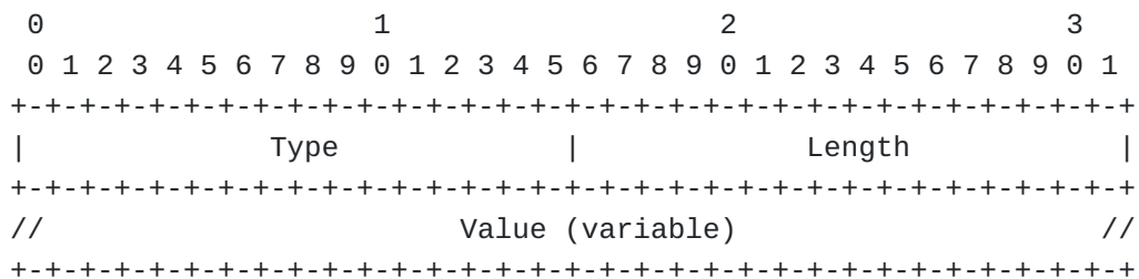
Figure 4: TLV Format
