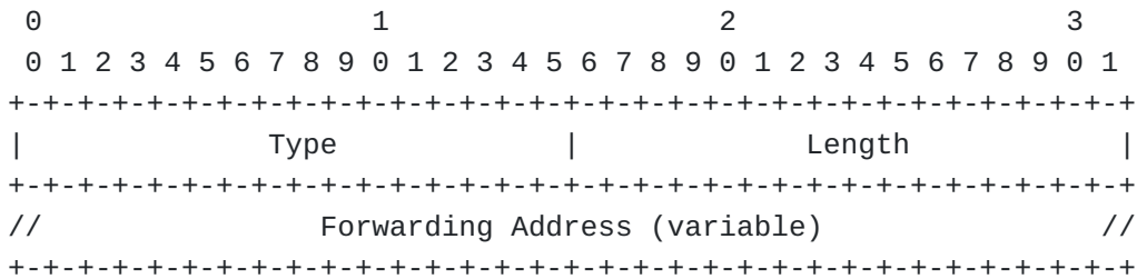
Figure 29: OSPF Forwarding Address TLV Format
