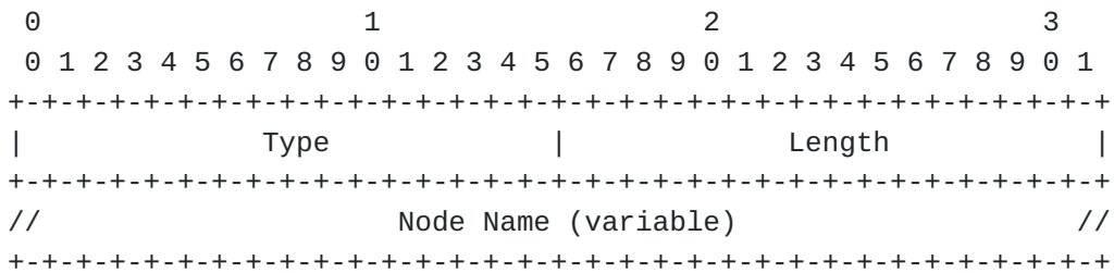
Figure 17: Node Name Format
