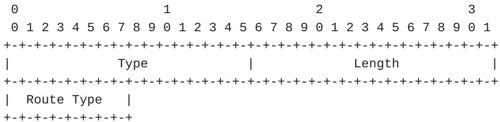
Figure 13: OSPF Route Type TLV Format
