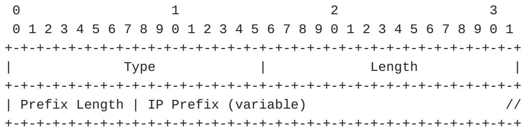
Figure 14: IP Reachability Information TLV Format
