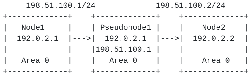
Figure 33: OSPF Pseudonodes
