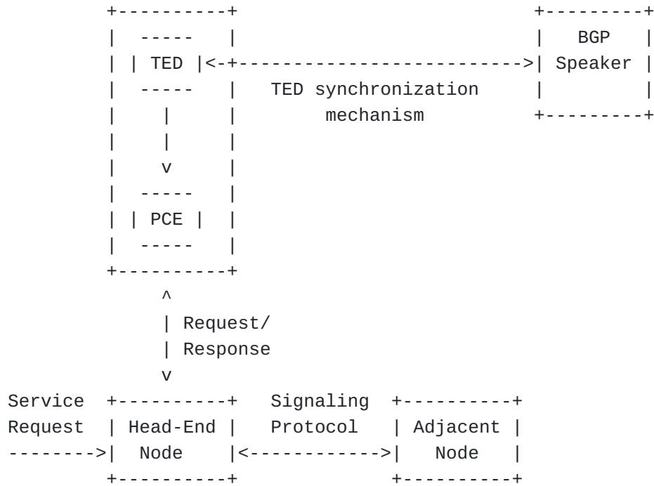
Figure 2: External PCE Node Using a TED Synchronization Mechanism
