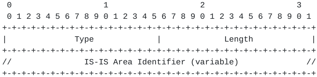
Figure 16: IS-IS Area Identifier TLV Format
