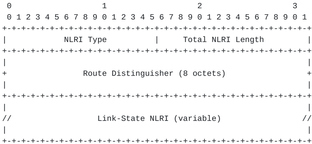
Figure 6: Link-State VPN AFI 16388 / SAFI 72 NLRI Format
