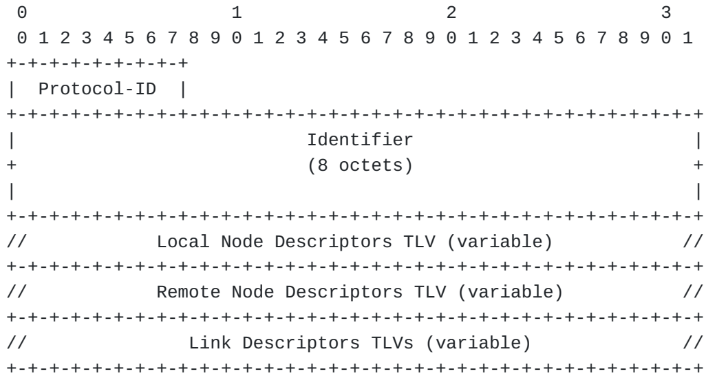
Figure 8: The Link NLRI Format
