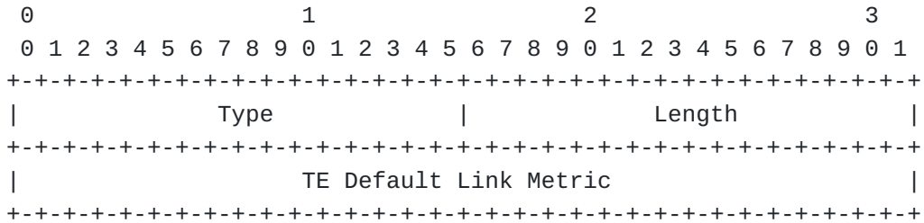
Figure 20: TE Default Metric TLV Format
