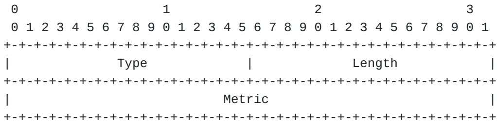
Figure 28: Prefix Metric TLV Format
