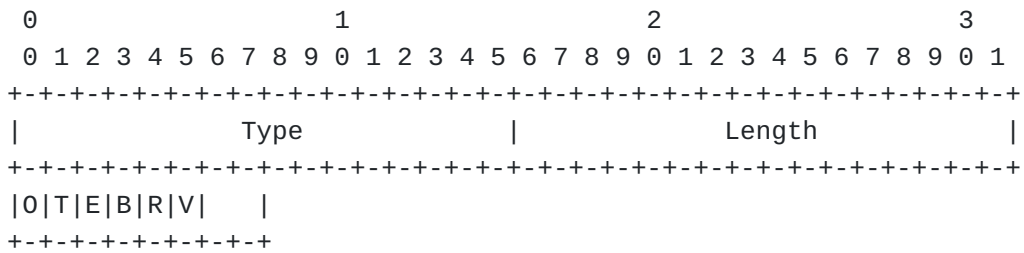
Figure 15: Node Flag Bits TLV Format
