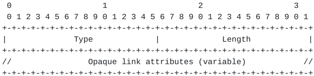
Figure 23: Opaque Link Attribute TLV Format
