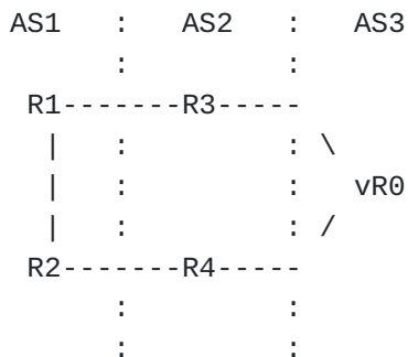
Figure 36: Multi-AS Aggregation
