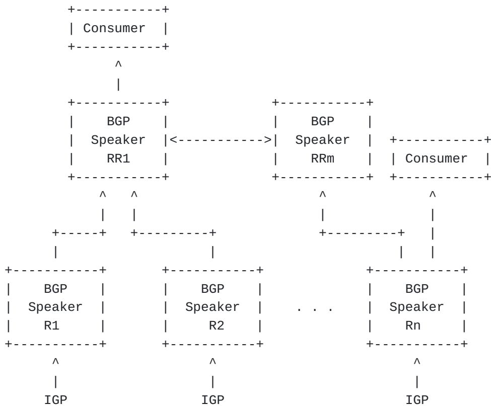
Figure 1: Collection of Link-State and TE Information
