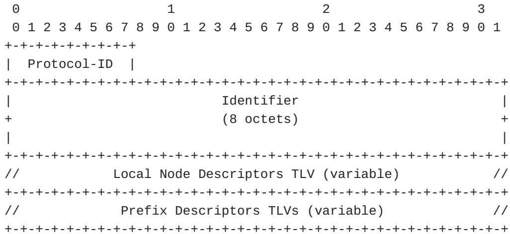
Figure 9: The IPv4/IPv6 Topology Prefix NLRI Format
