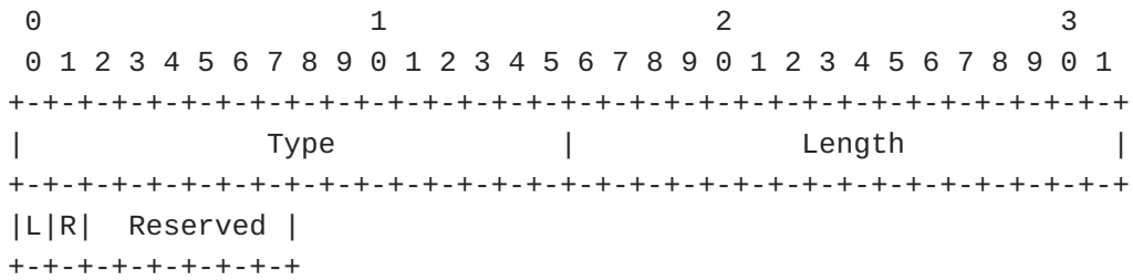
Figure 19: MPLS Protocol Mask TLV
