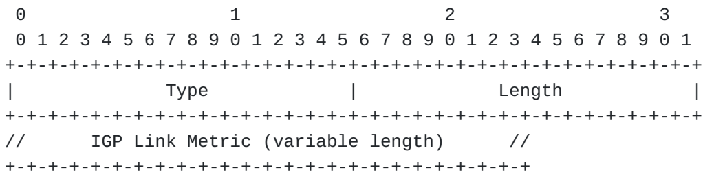
Figure 21: IGP Metric TLV Format
