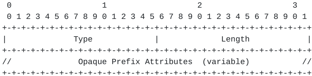
Figure 30: Opaque Prefix Attribute TLV Format
