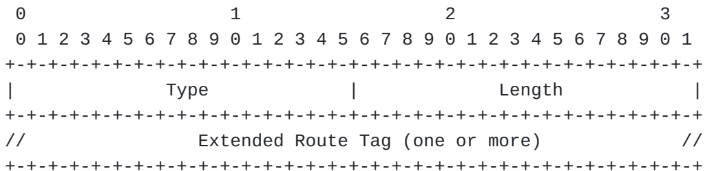
Figure 27: Extended IGP Route Tag TLV Format
