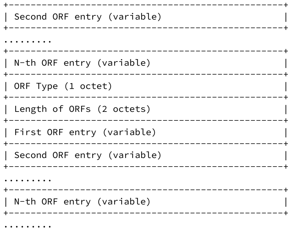
Fig 1. Carrying ORF entries in the ROUTE-REFRESH message
