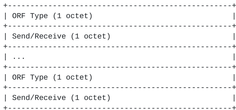
Fig 4. Capability encoding
