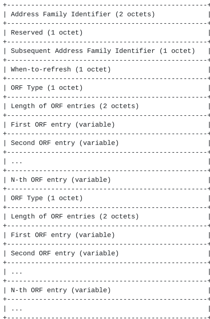
Figure 1: Carrying ORF Entries in the ROUTE-REFRESH Message
