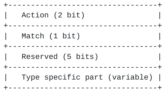
Figure 2: ORF Entry Encoding
