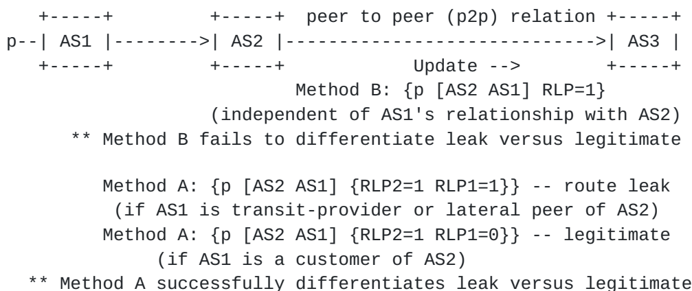
Figure 3: Illustration of the basic notion of a route leak.
