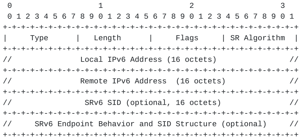
Figure 21: Type K Segment sub-TLV
