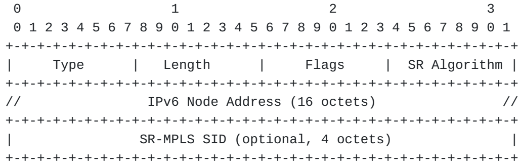
Figure 14: Type D Segment sub-TLV
