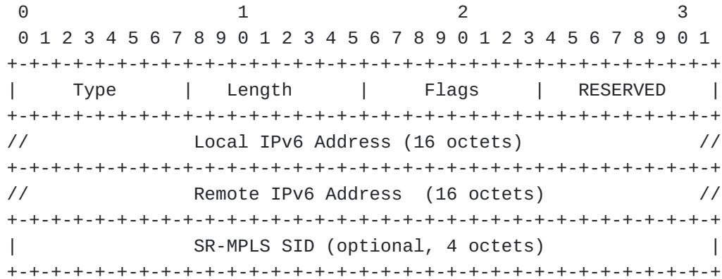
Figure 18: Type H Segment sub-TLV
