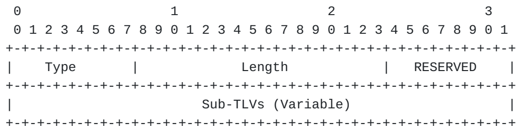
Figure 3. SR Reverse Path Segment List Sub-TLV
