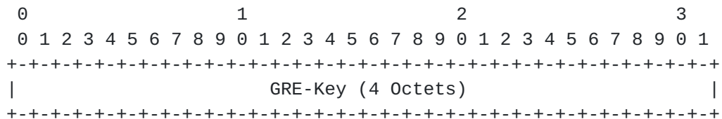
Figure 10: MPLS-in-GRE Encapsulation Sub-TLV
