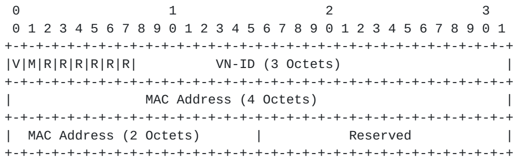
Figure 6: NVGRE Encapsulation Sub-TLV
