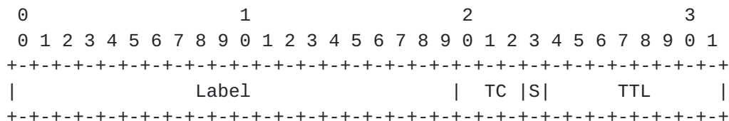
Figure 11: MPLS Label Stack Sub-TLV
