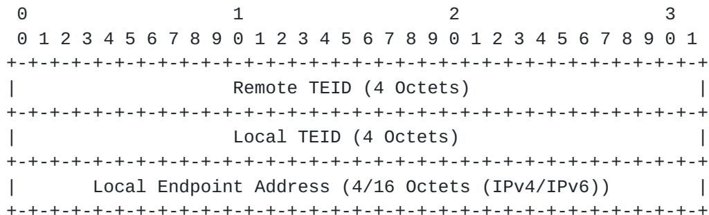
Figure 8: GTP Encapsulation Sub-TLV
