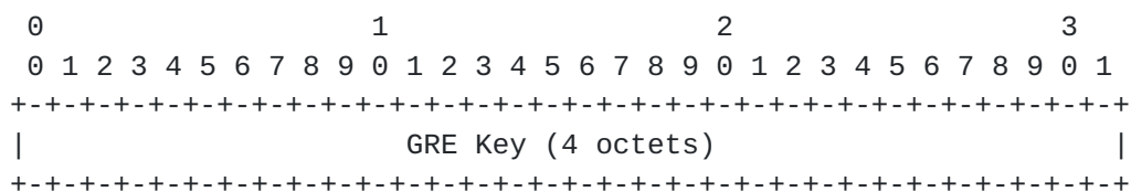
Figure 9: GRE Encapsulation Sub-TLV
