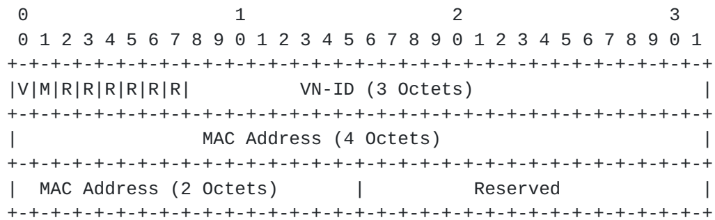
Figure 4: VXLAN Encapsulation Sub-TLV
