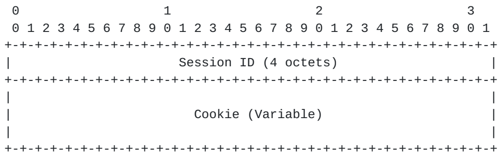
Figure 6: L2TPv3 Encapsulation Sub-TLV
