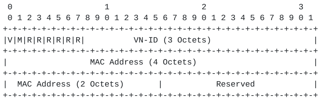
Figure 5: NVGRE Encapsulation Sub-TLV
