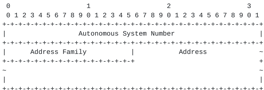
Figure 2: Remote Endpoint Sub-TLV Value Field
